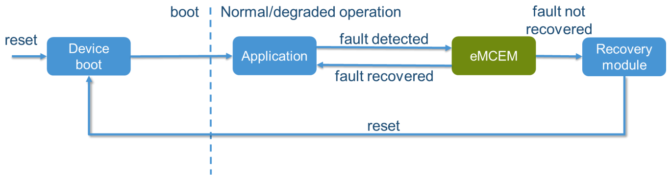
Figure 3. eMCEM (extended Microcontroller Error Manager)
