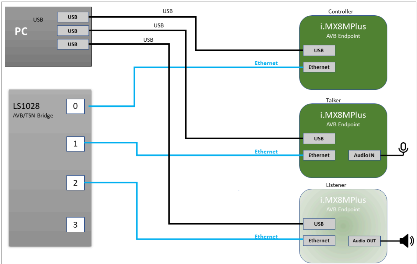
Figure 17. Harpoon AVTP Talker/Listener setup
