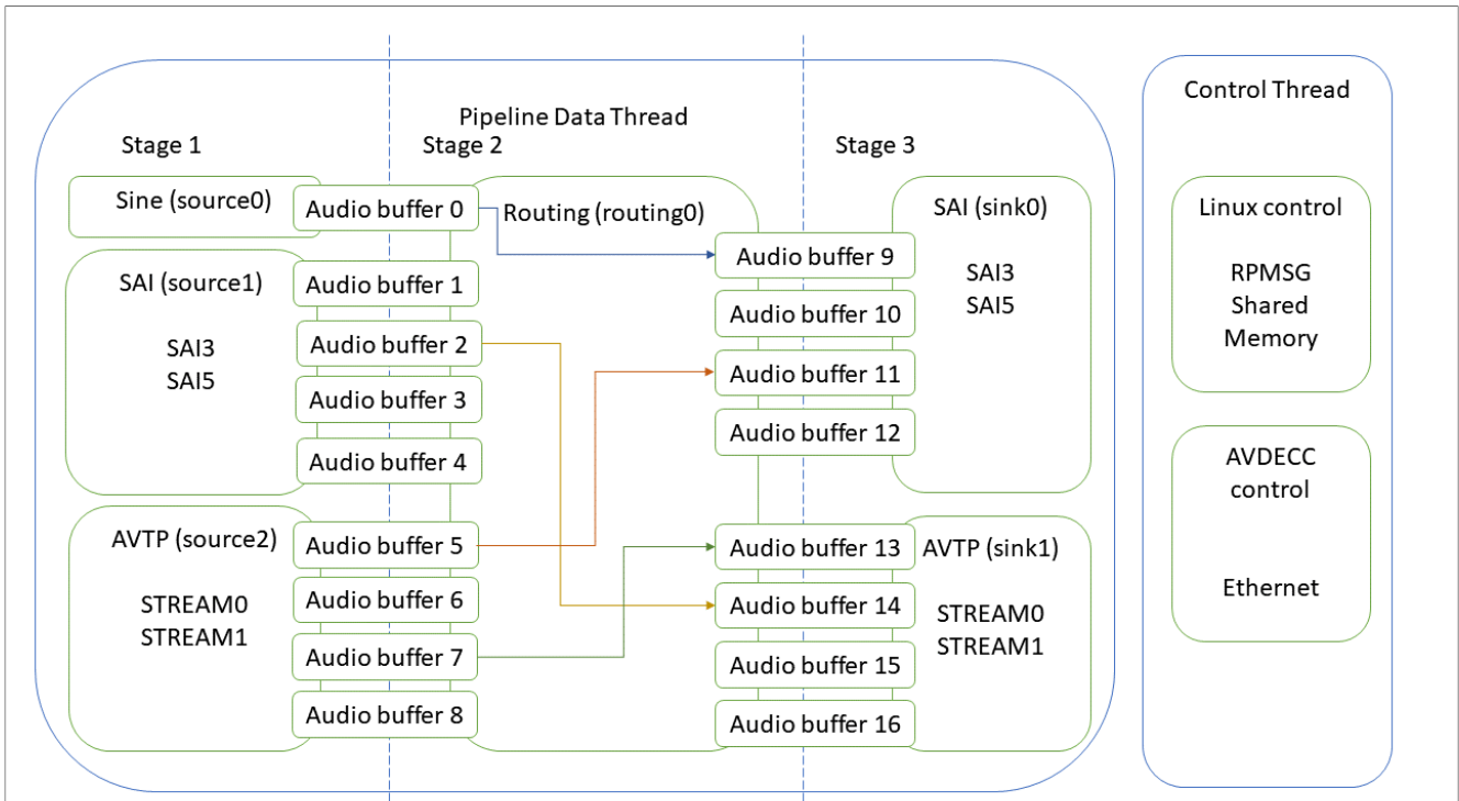
AVB Audio pipeline showing the AVTP Listener with multiple streams as a source.
