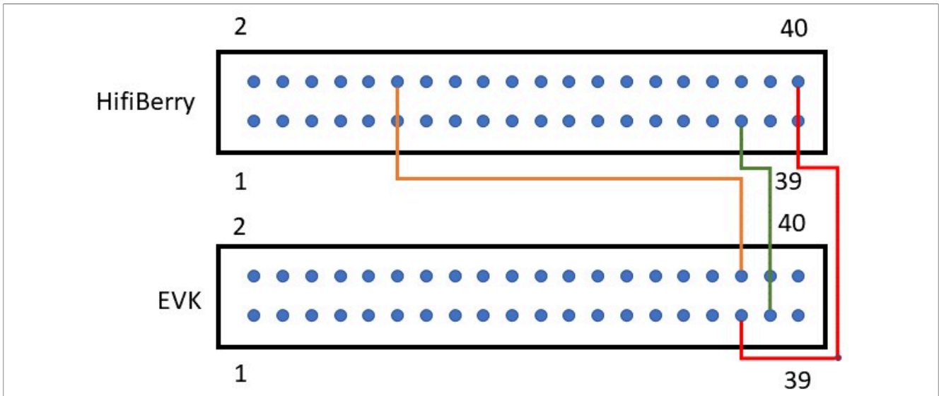
Figure 7. Transposer (Top View)
