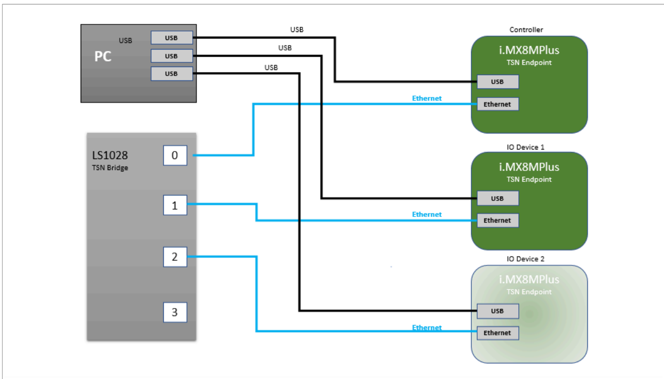
Figure 19. TSN endpoint sample application setup
