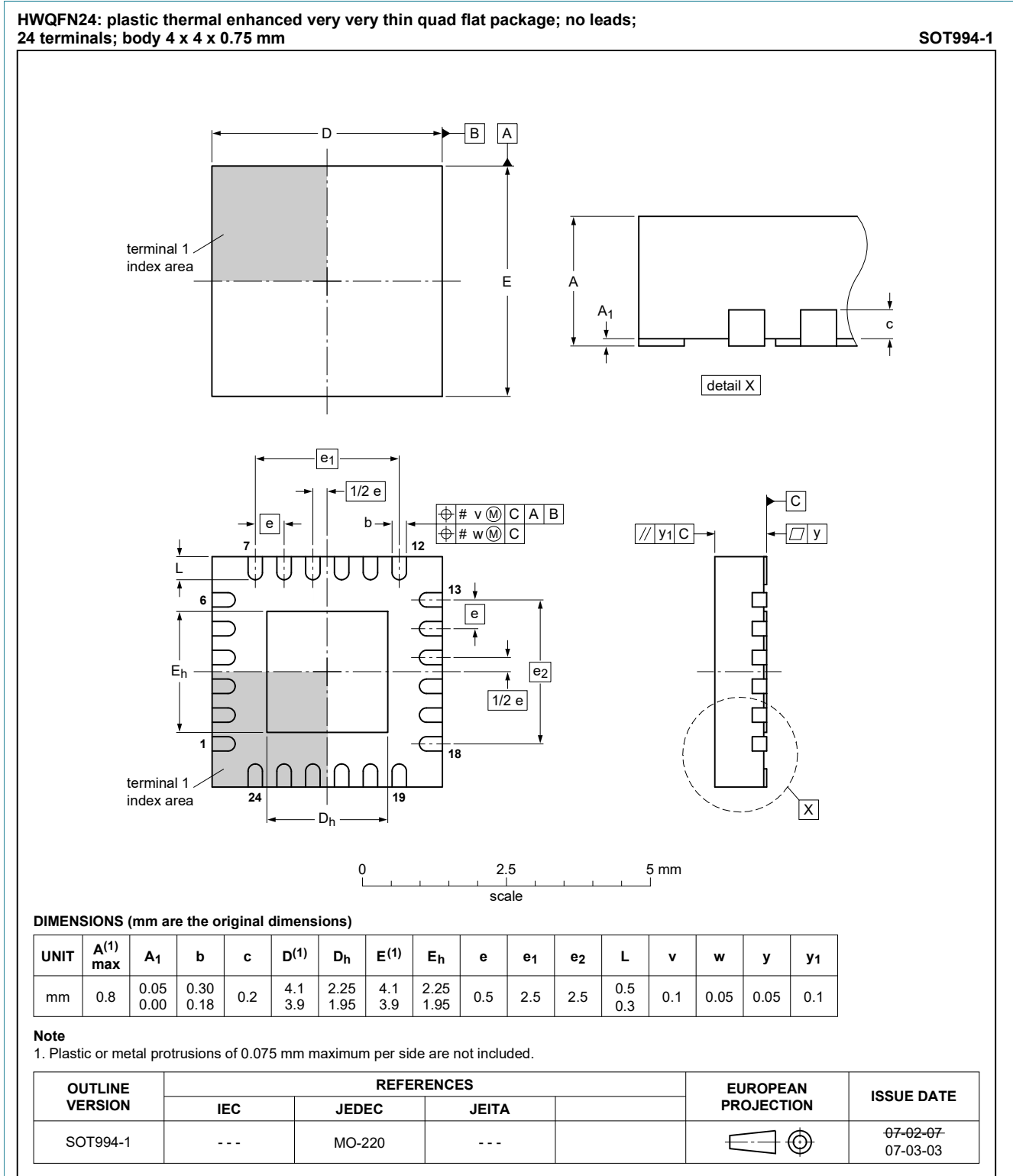
Figure 1. Package outline HWQFN24 (SOT994-1)
