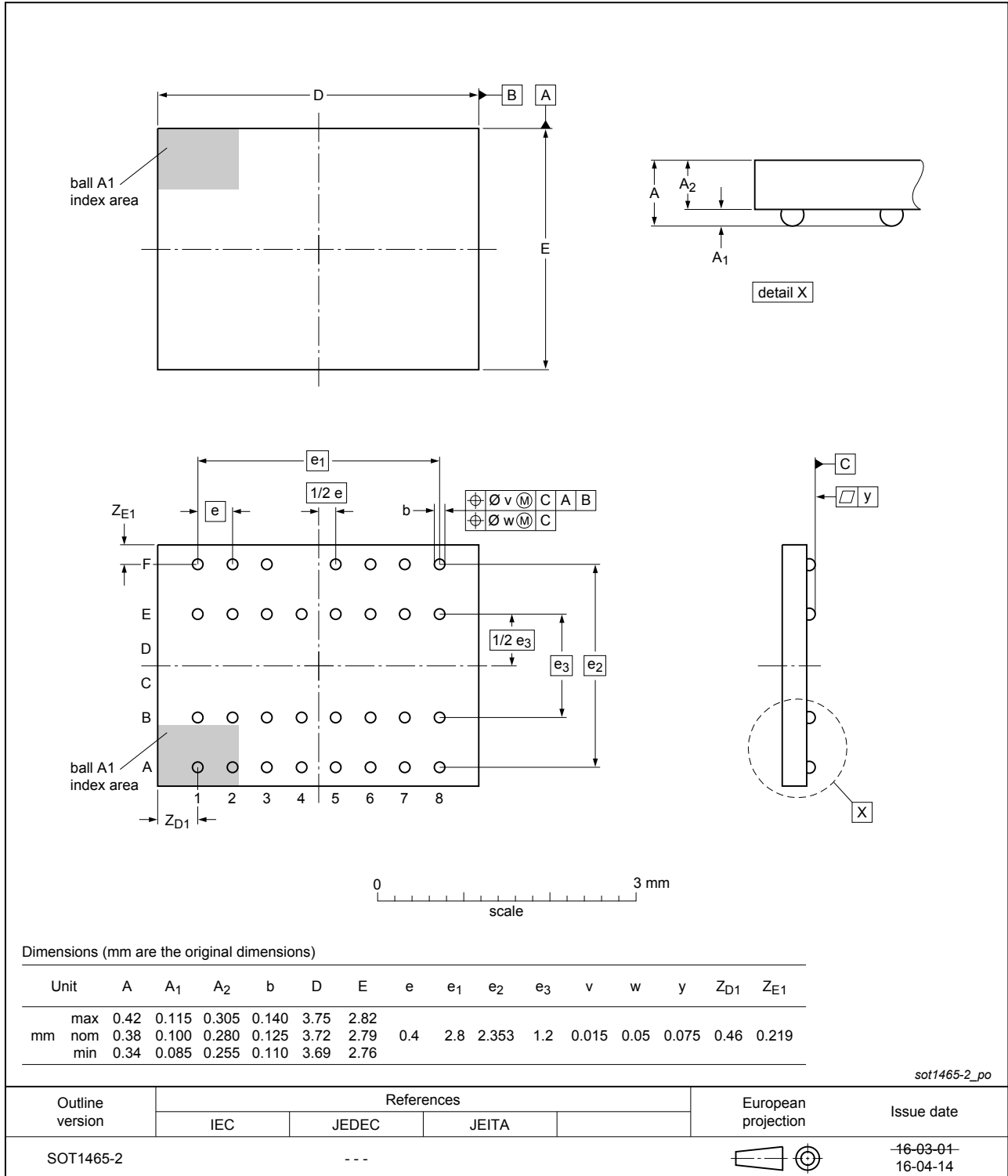
Fig. 1. Package outline WLCSP31 (SOT1465-2)
