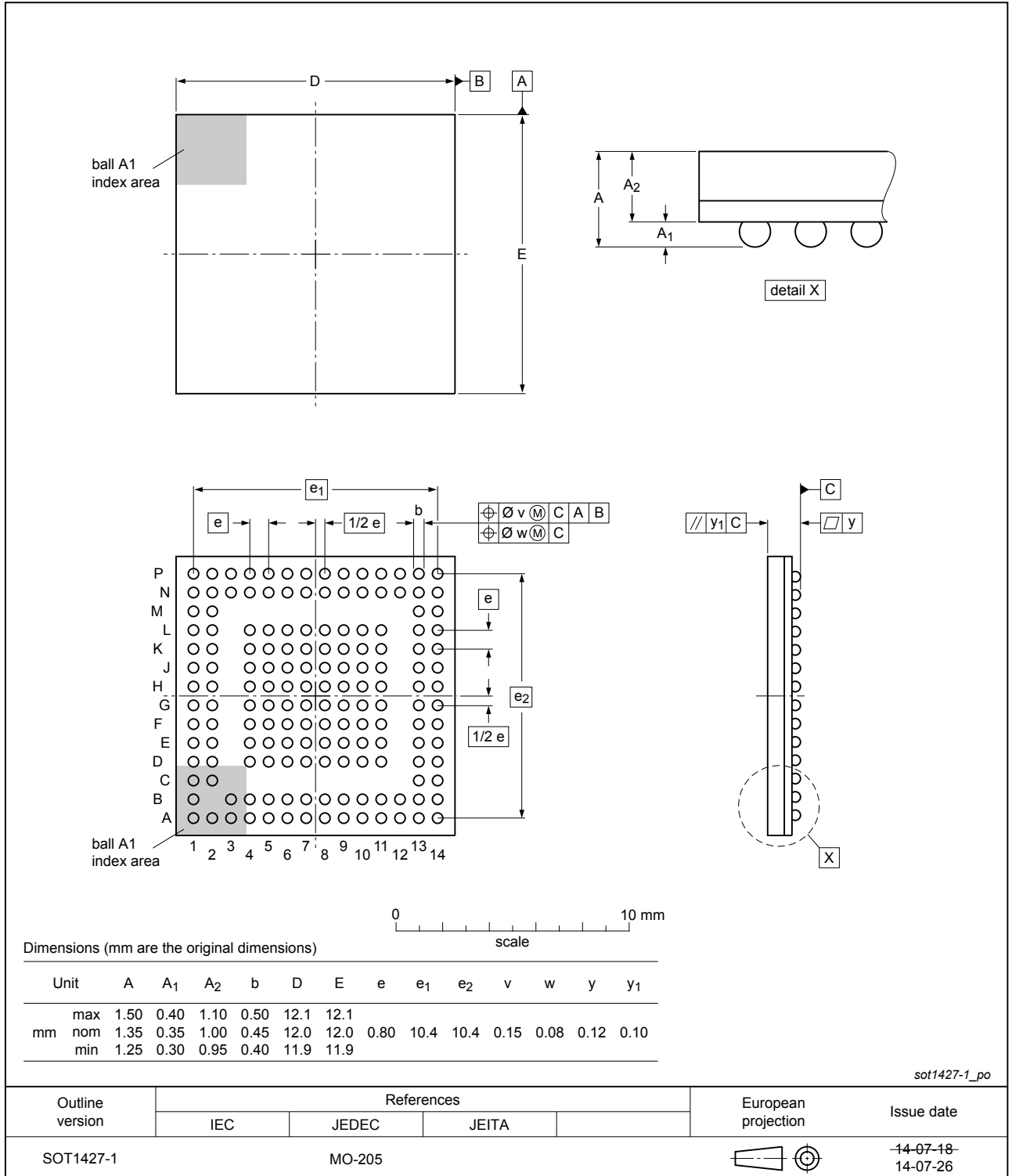
Fig. 1. Package outline LFBGA159 (SOT1427-1)
