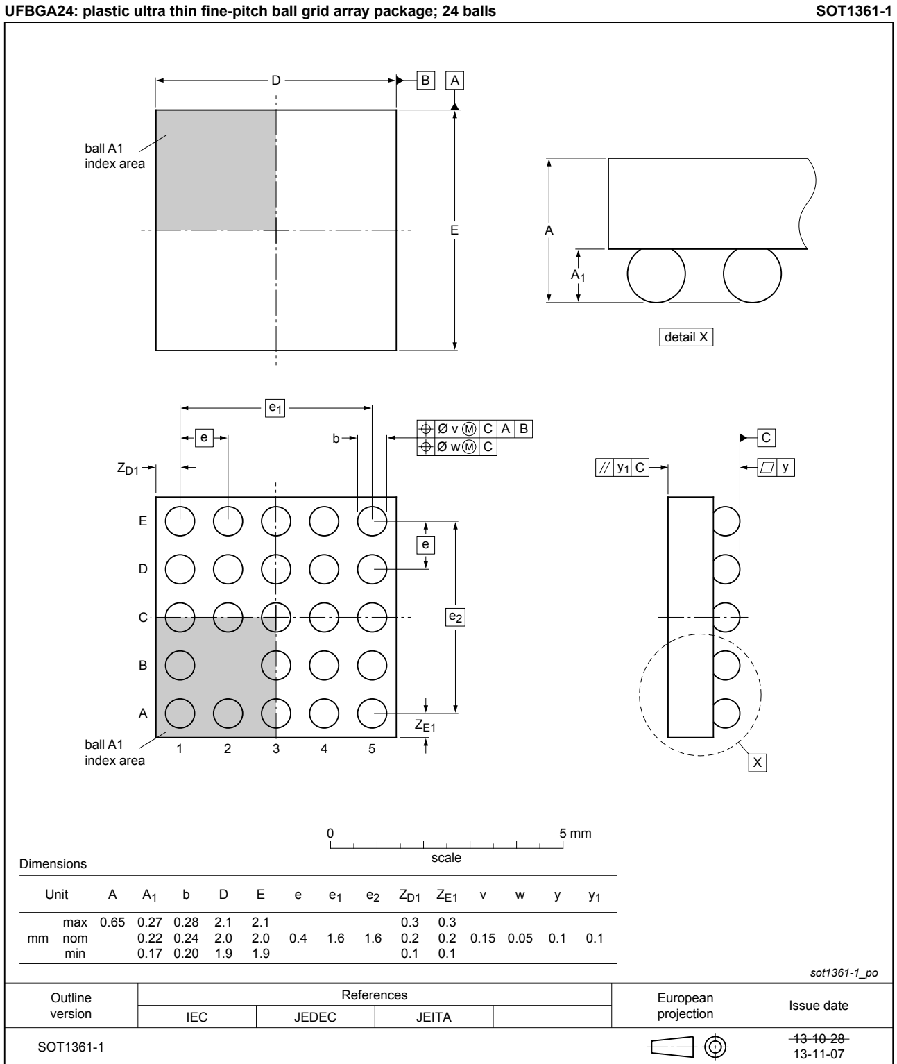
Fig. 1. Package outline UFBGA24 (SOT1361-1)
