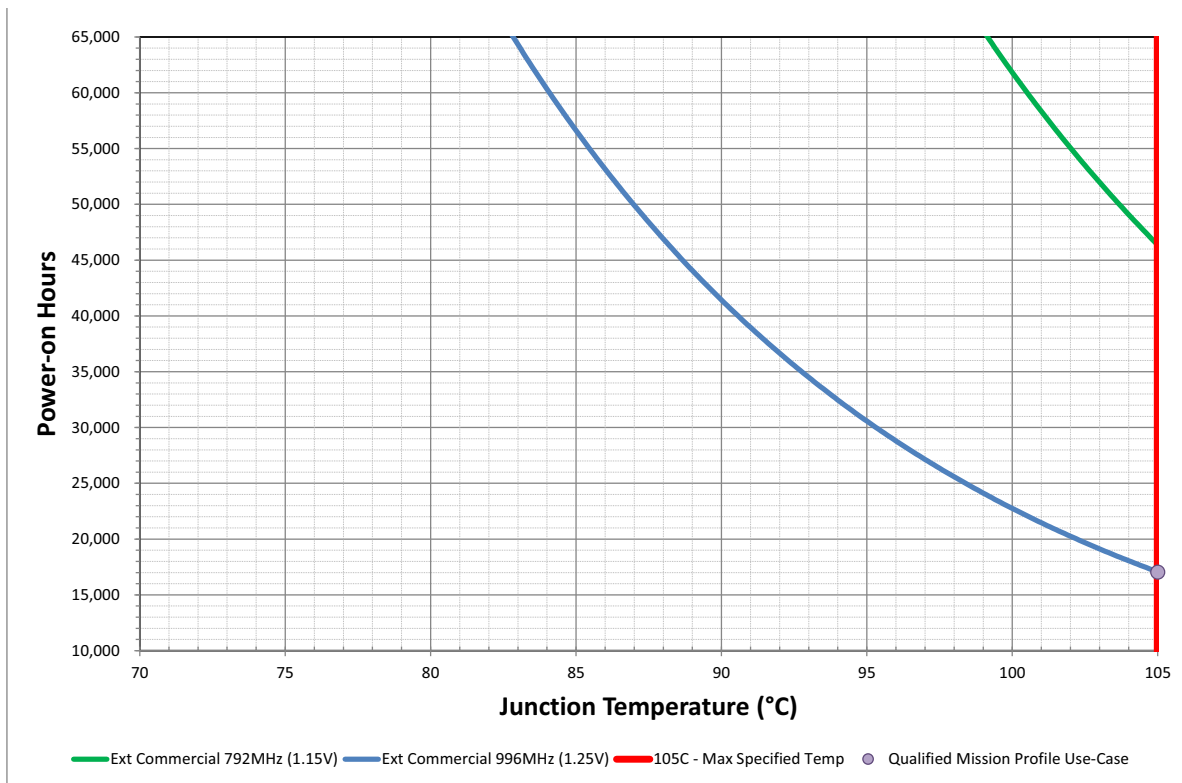
Figure 3. i.MX 6SoloLite extended commercial lifetime estimates LDO enabled mode
