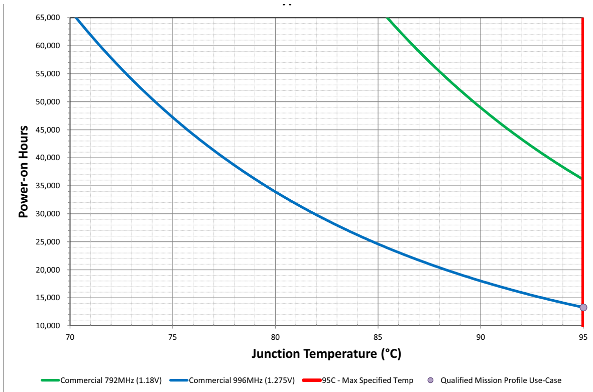
Figure 2. i.MX 6SoloLite commercial lifetime estimates LDO bypass mode
