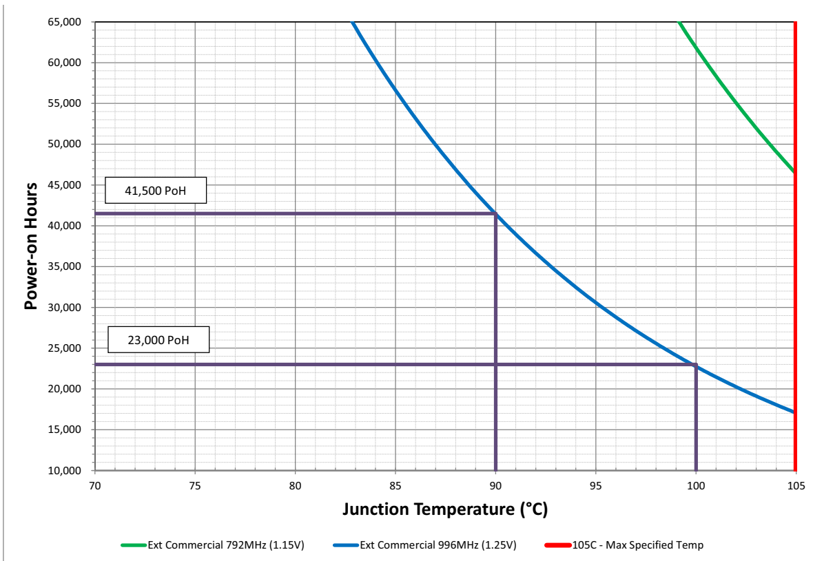
Figure 6. Multiple temperature use case
