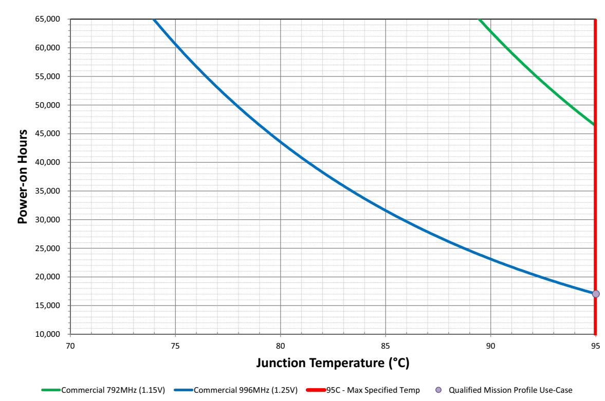
Figure 1. i.MX 6SoloLite commercial lifetime estimates LDO enabled mode
