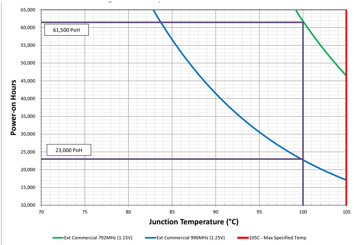
Figure 5. Multiple power state use case
