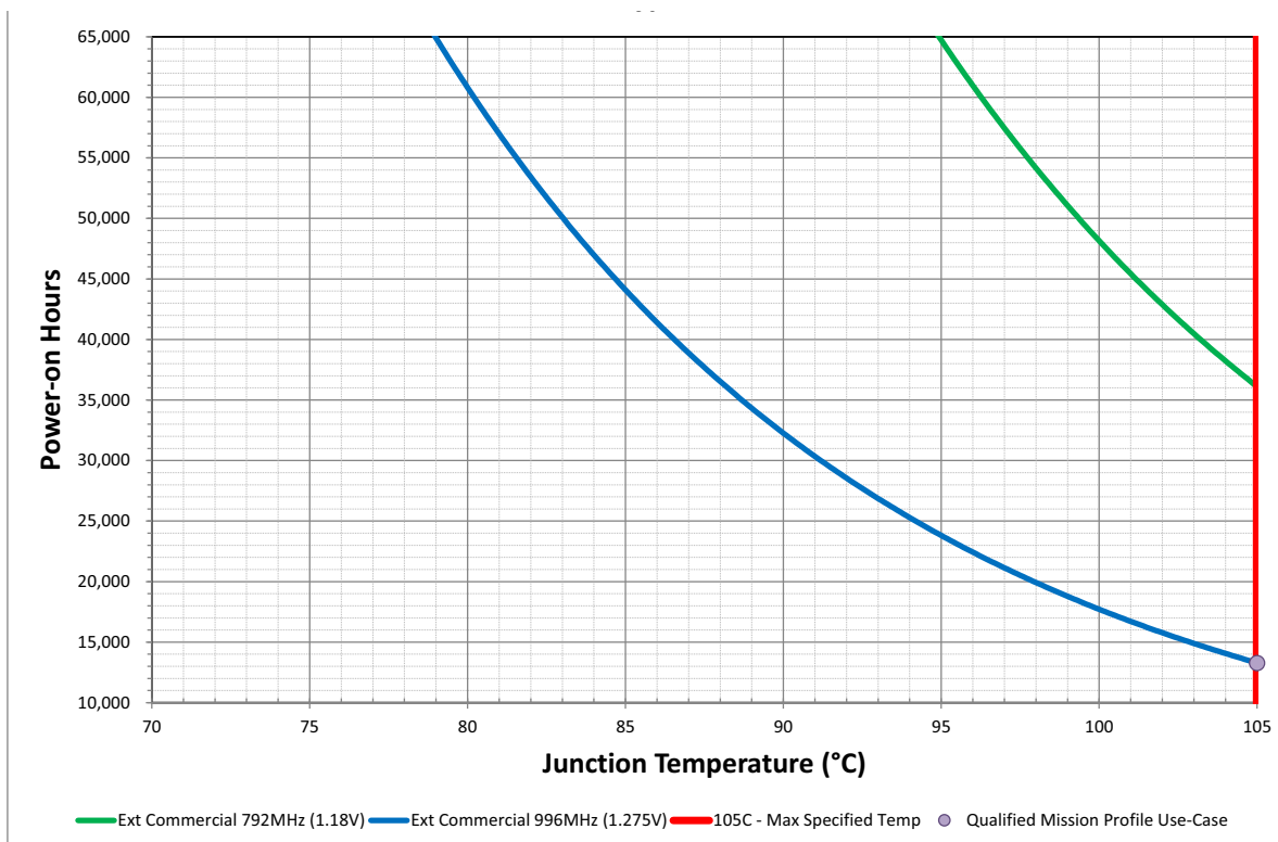
Figure 4. i.MX 6SoloLite extended commercial lifetime estimates LDO bypass mode
